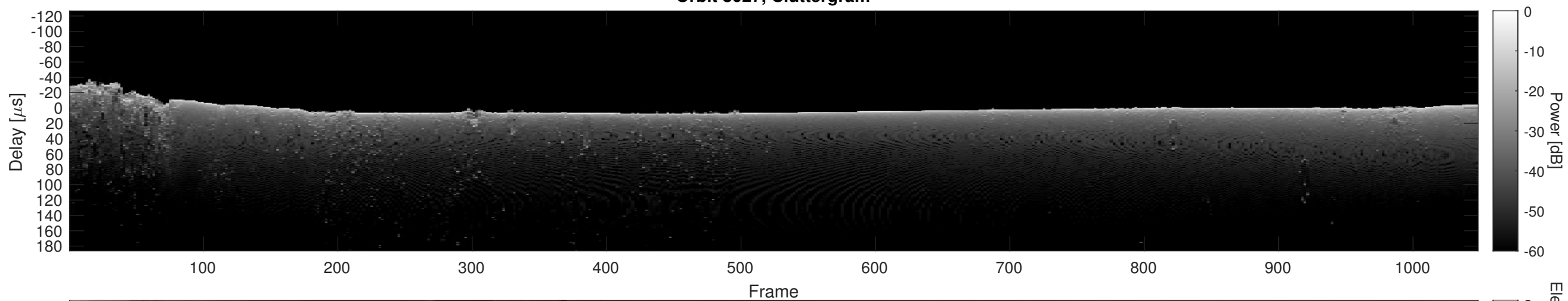
Orbit 8027, Cluttergram
