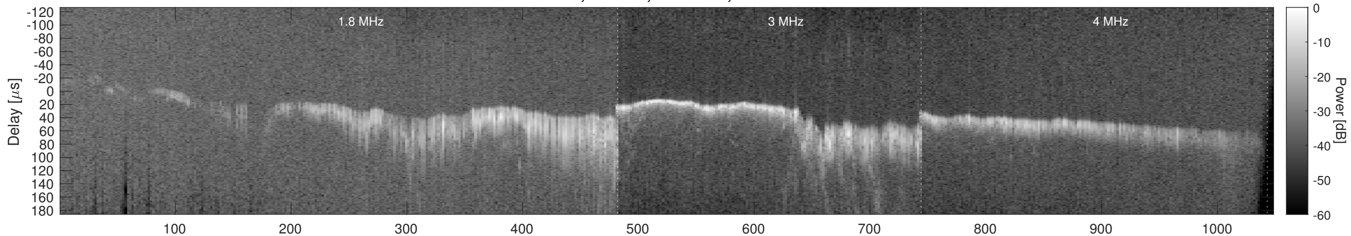
Orbit 8027, Window, Channel 2, Chapman
