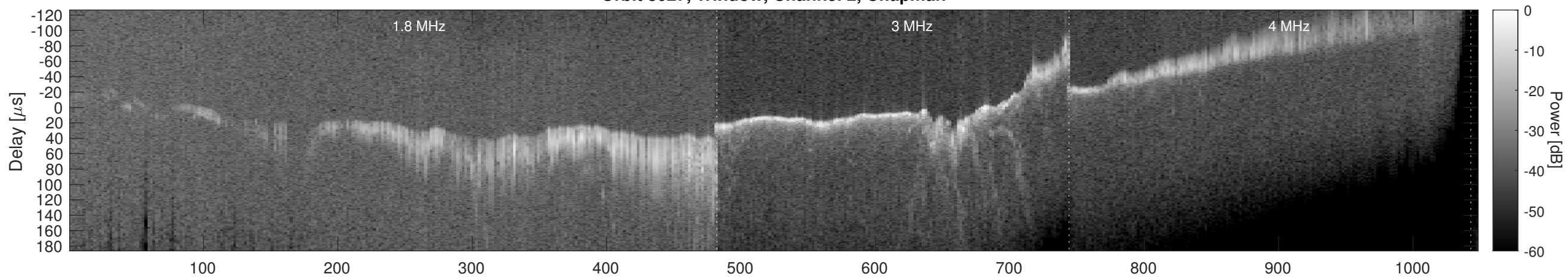
Orbit 8027, Window, Channel 2, Optimized
