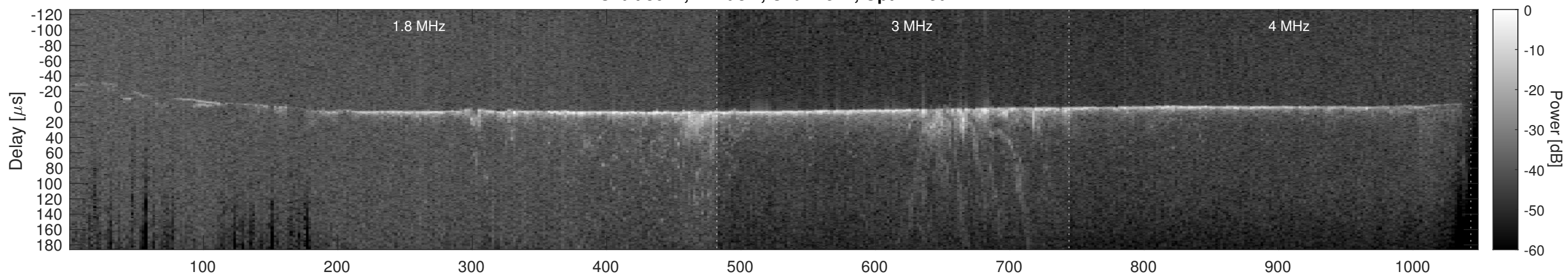
Orbit 8027, Cluttergram
