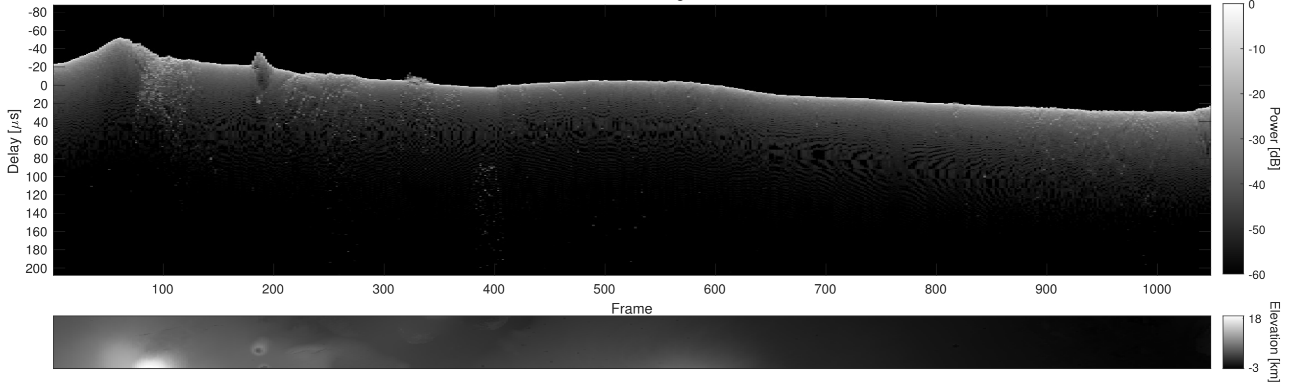
Orbit 8030, Cluttergram
