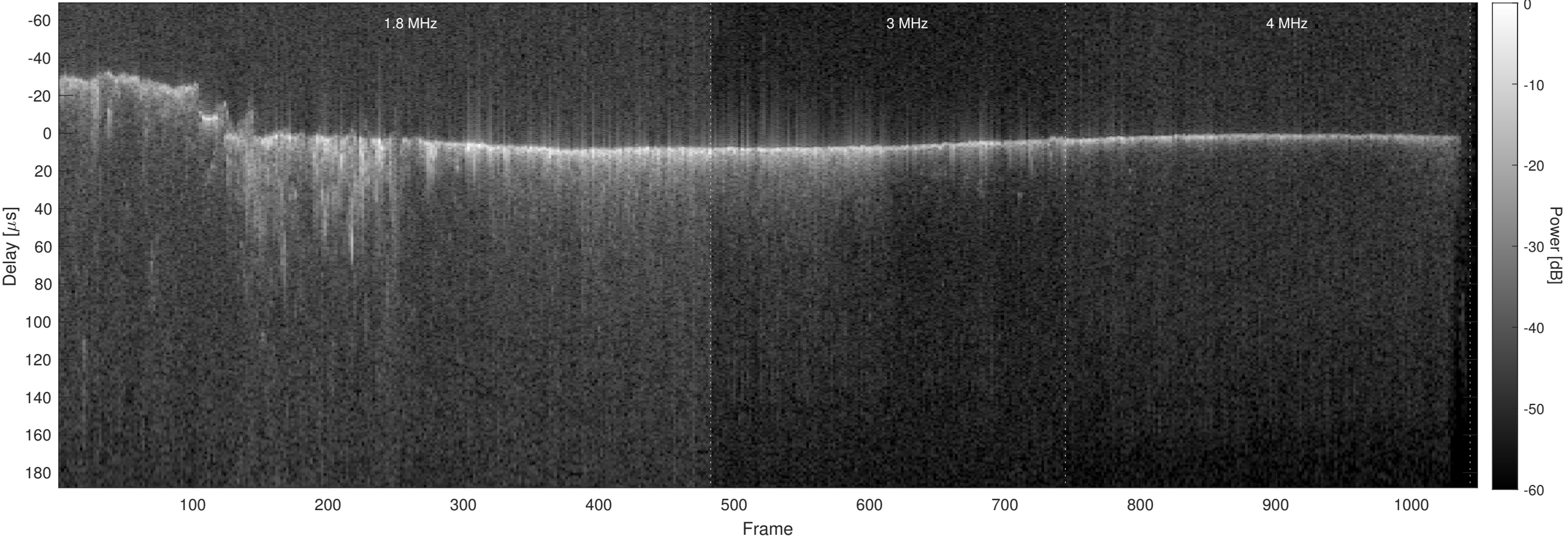
Orbit 8031, Optimized, No Window, Channel 2
