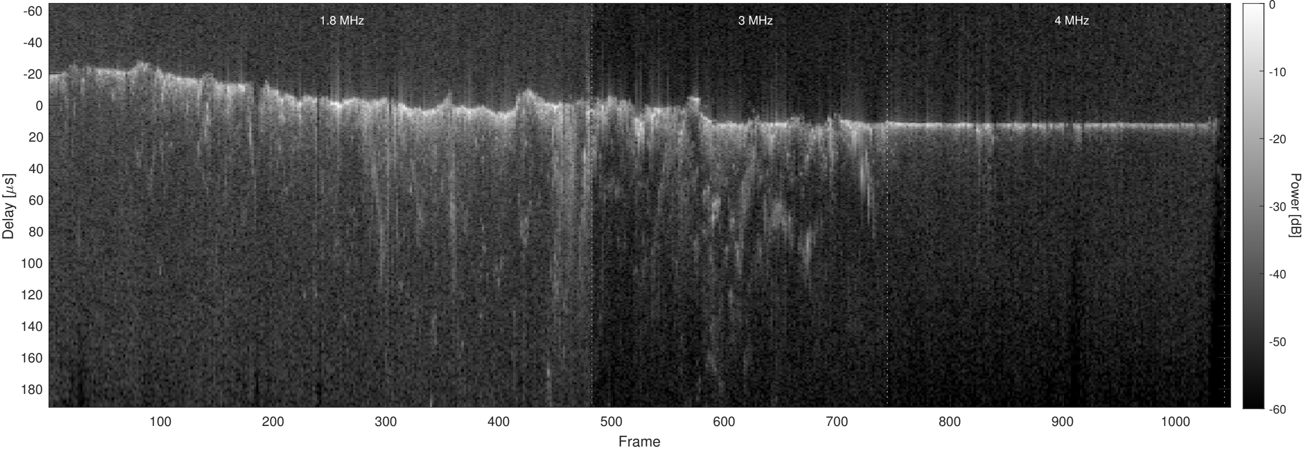
Orbit 8032, Optimized, No Window, Channel 2
