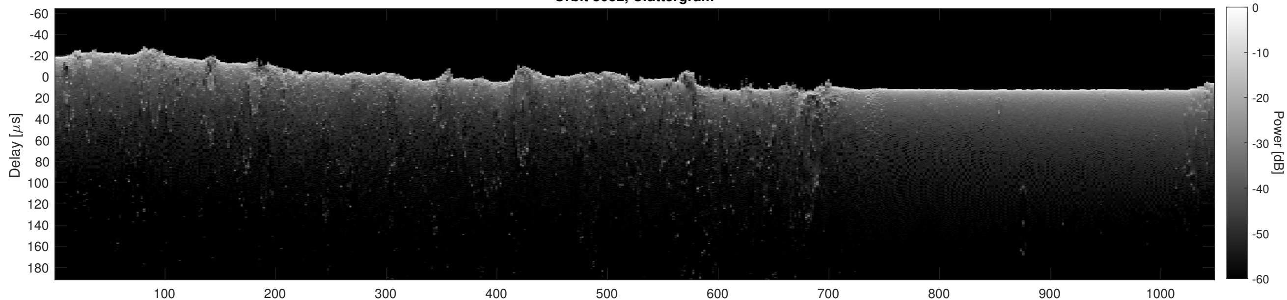
Orbit 8032, Cluttergram
