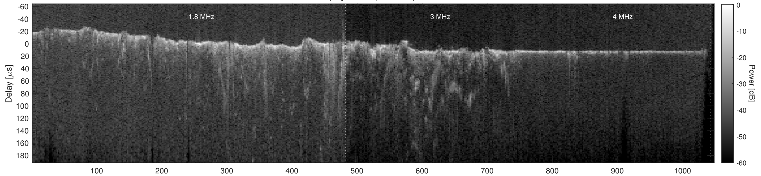
Orbit 8032, Cluttergram
