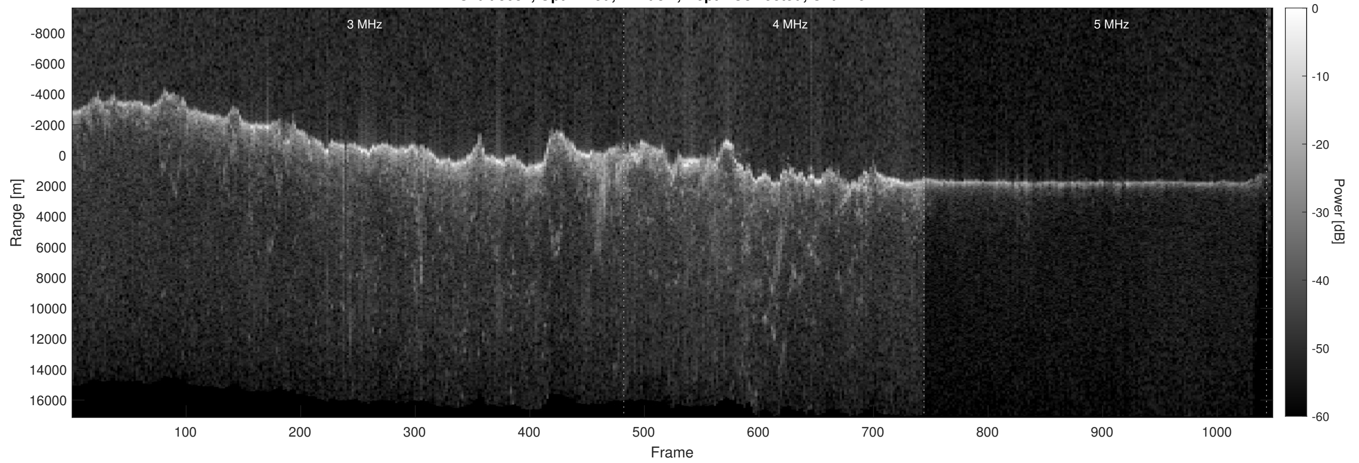
Orbit 8032, Optimized, Window, Depth-Corrected, Channel 2
