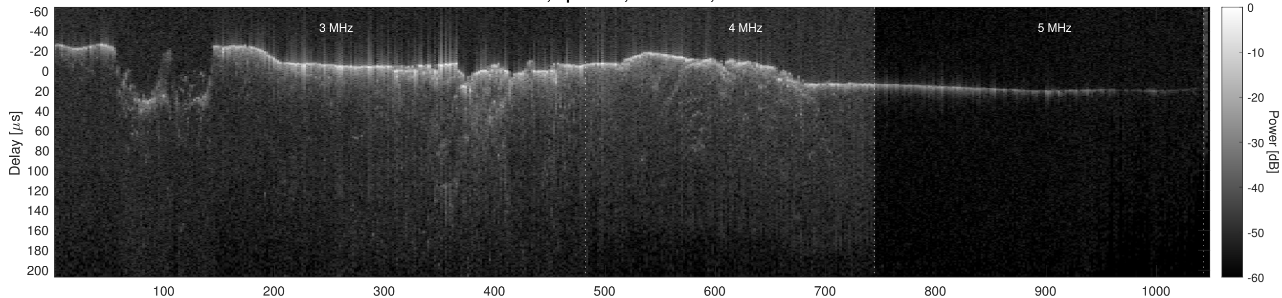
Orbit 8033, Optimized, No Window, Channel 2
