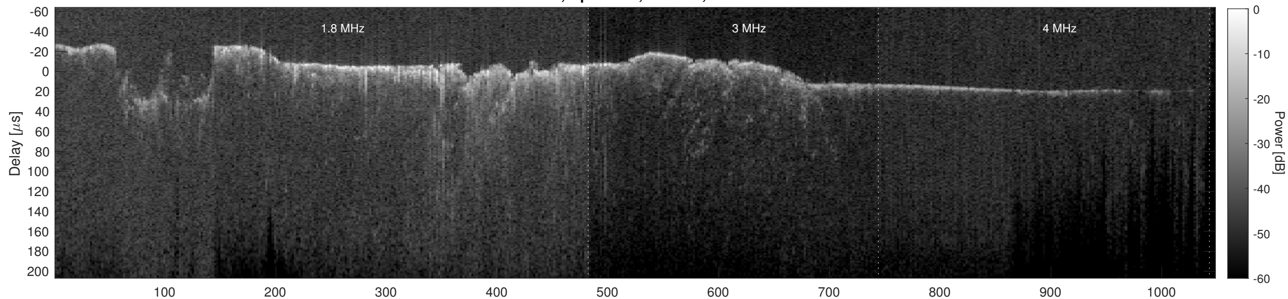
Orbit 8033, Cluttergram
