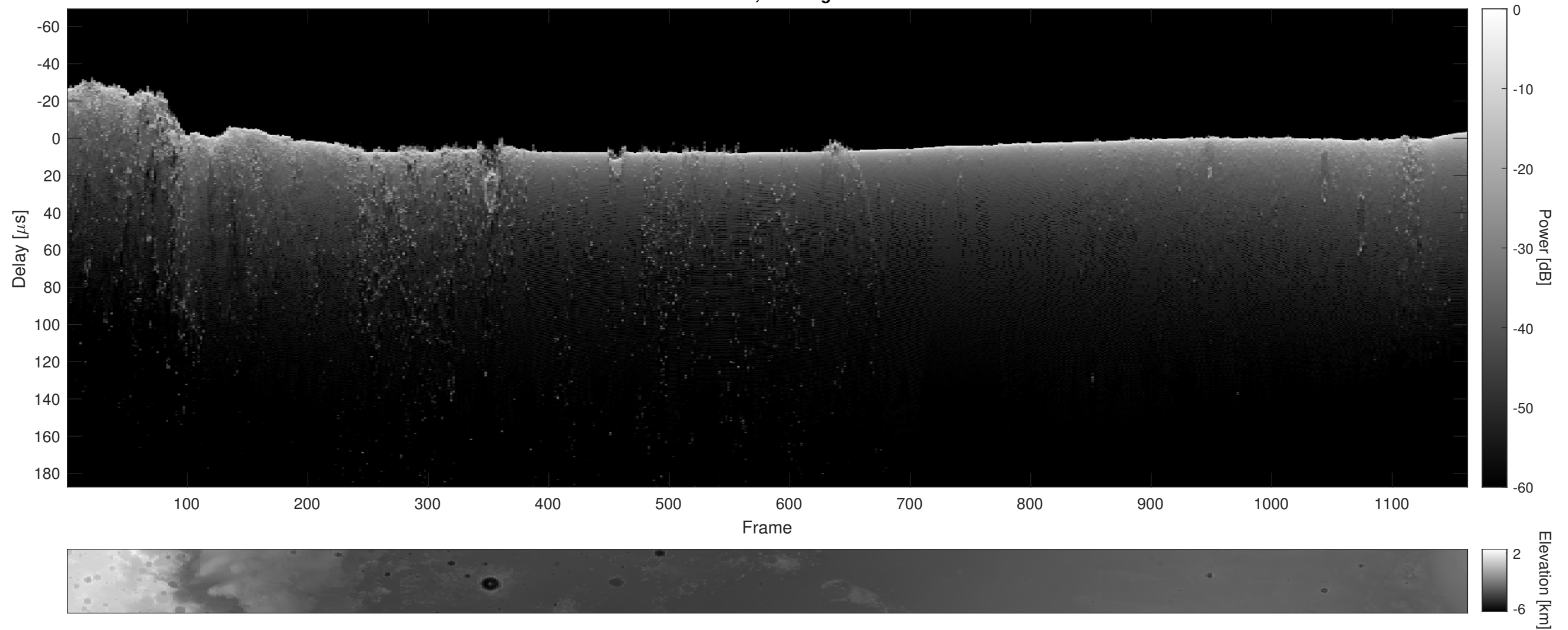
Orbit 8034, Cluttergram
