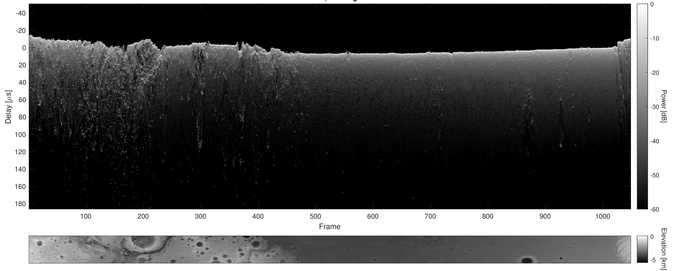
Orbit 8036, Cluttergram
