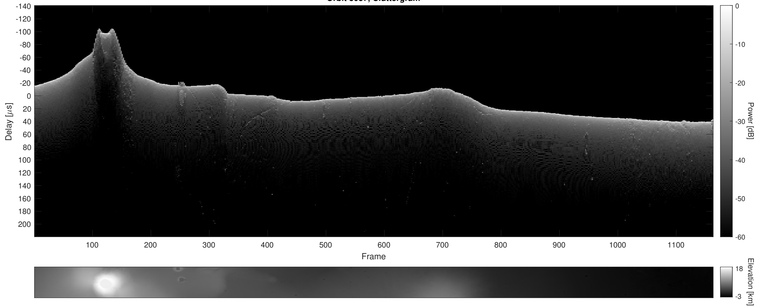
Orbit 8037, Cluttergram
