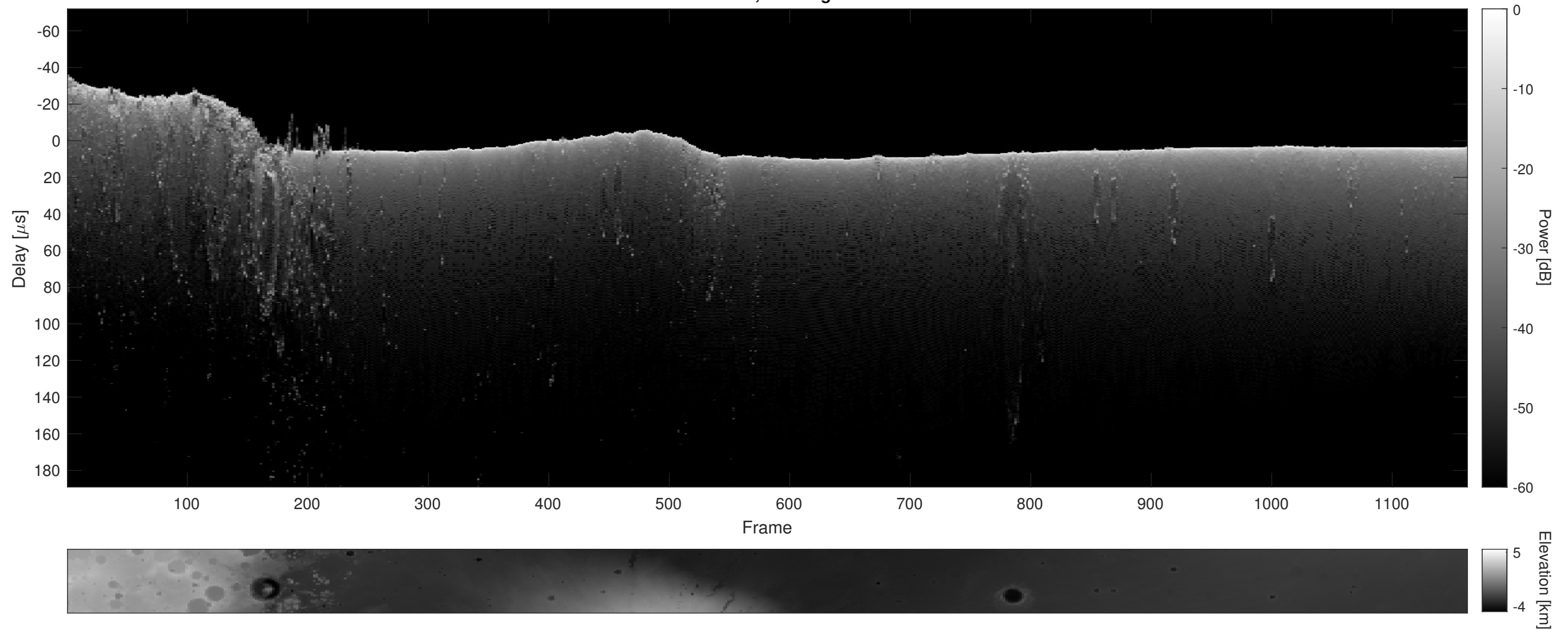
Orbit 8038, Cluttergram
