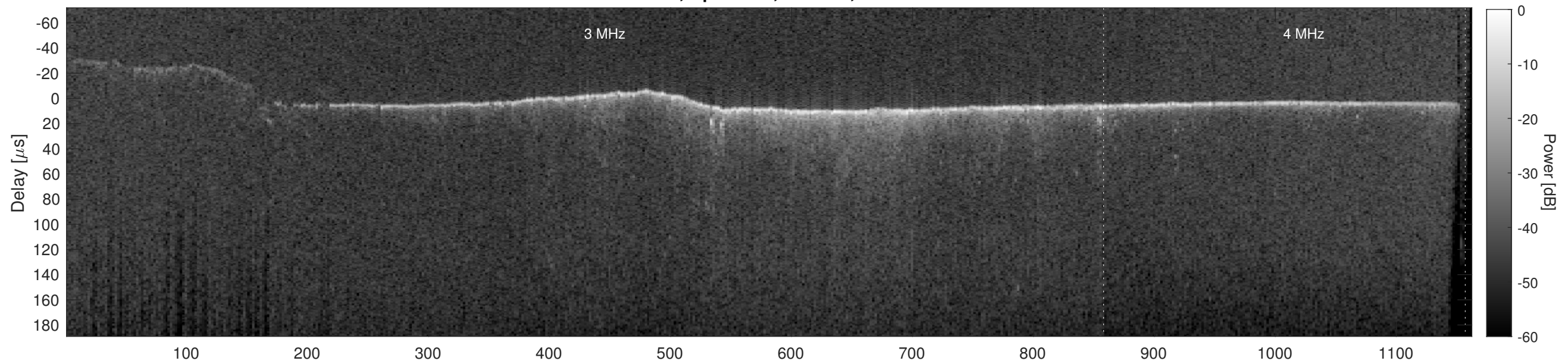
Orbit 8038, Cluttergram
