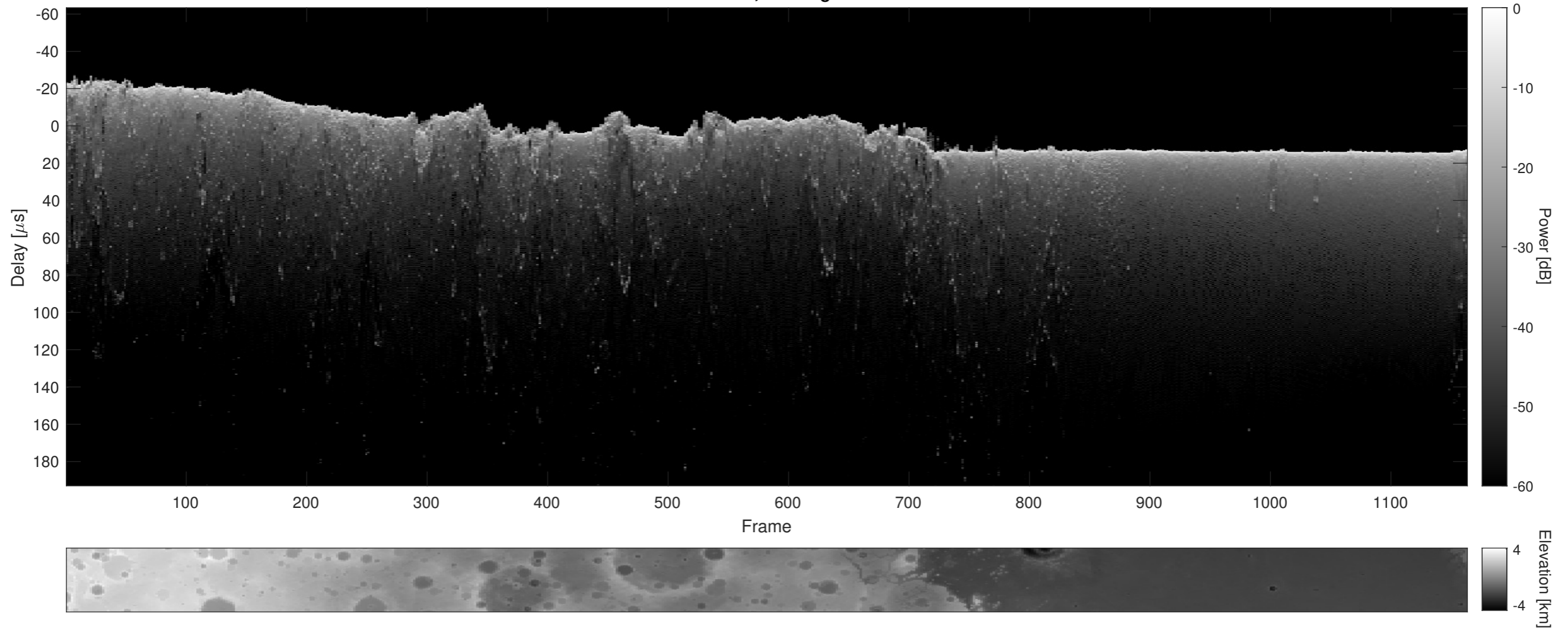
Orbit 8039, Cluttergram
