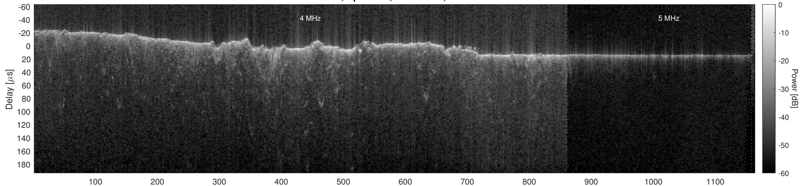
Orbit 8039, Optimized, No Window, Channel 2
