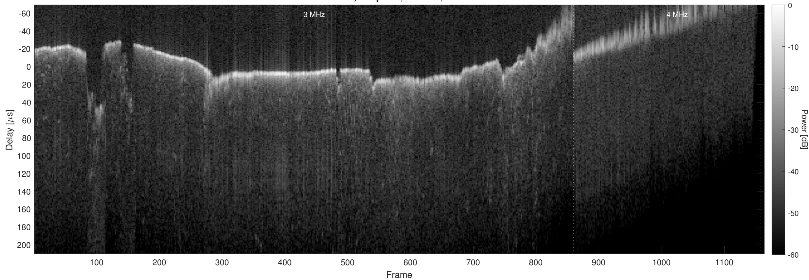
Orbit 8040, Chapman, Window, Channel 2
