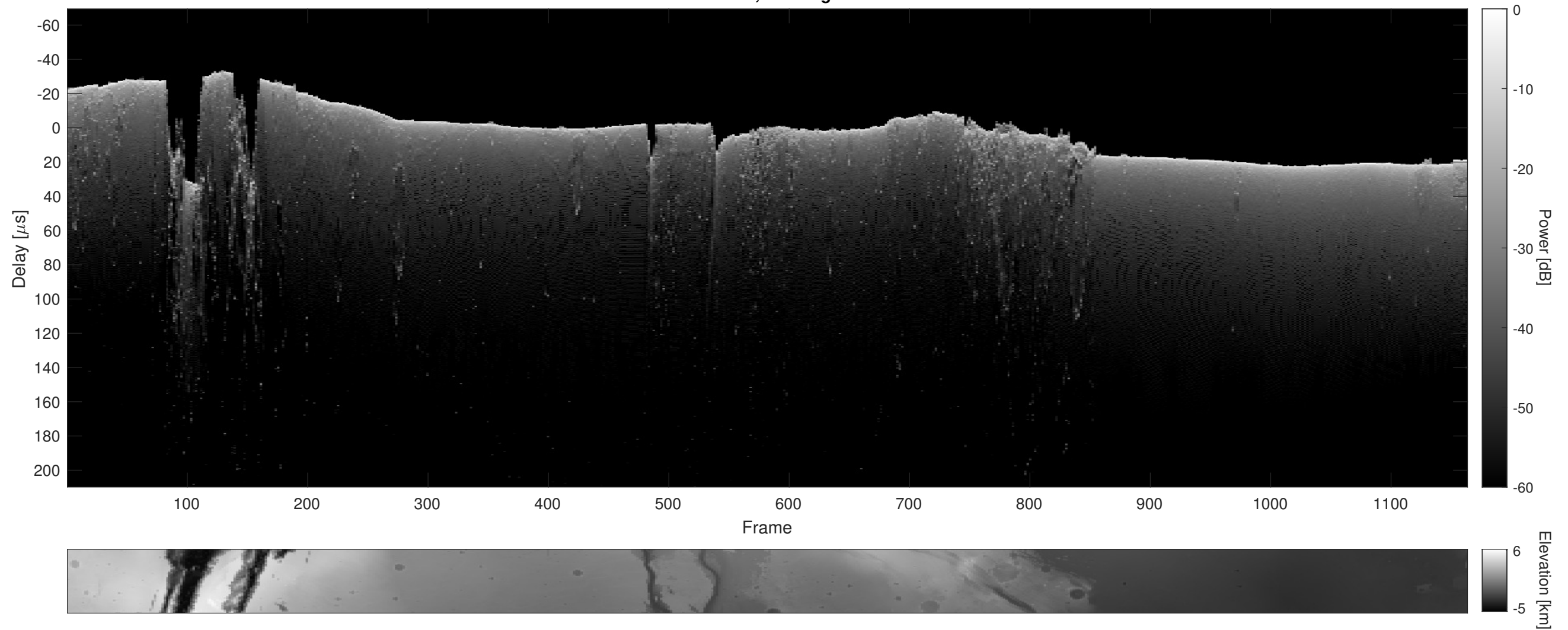
Orbit 8040, Cluttergram
