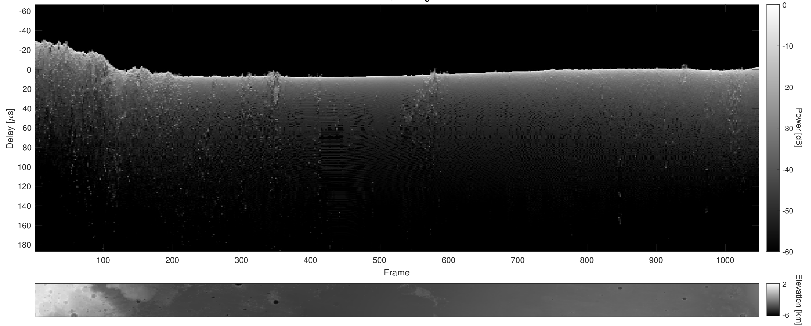
Orbit 8041, Cluttergram
