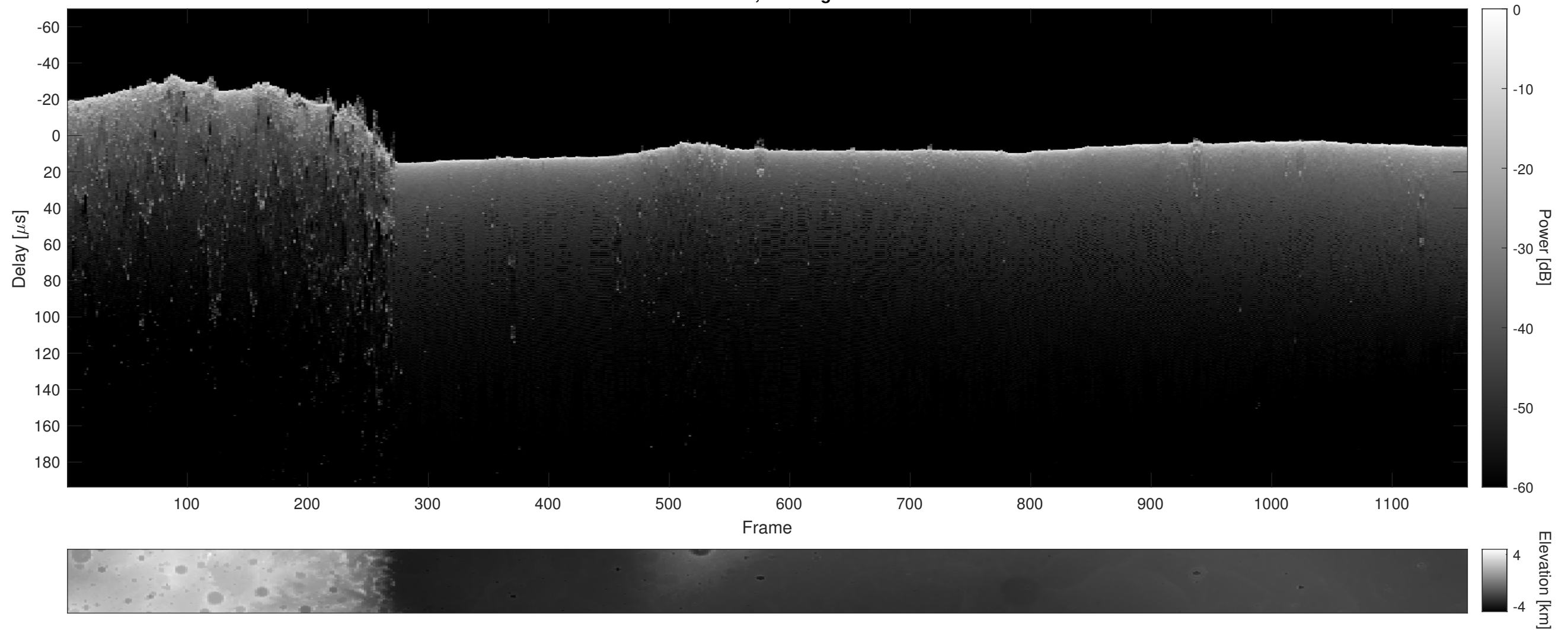
Orbit 8042, Cluttergram
