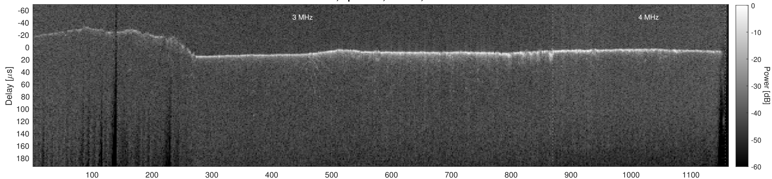
Orbit 8042, Cluttergram
