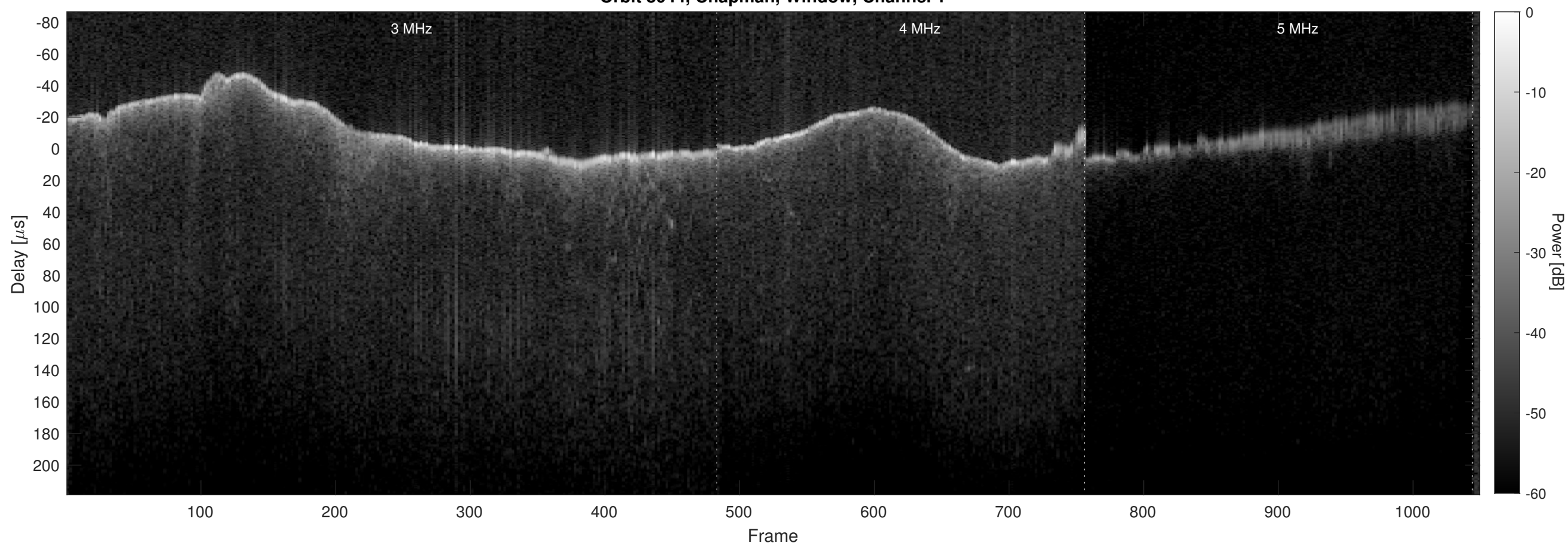
Orbit 8044, Chapman, Window, Channel 2
