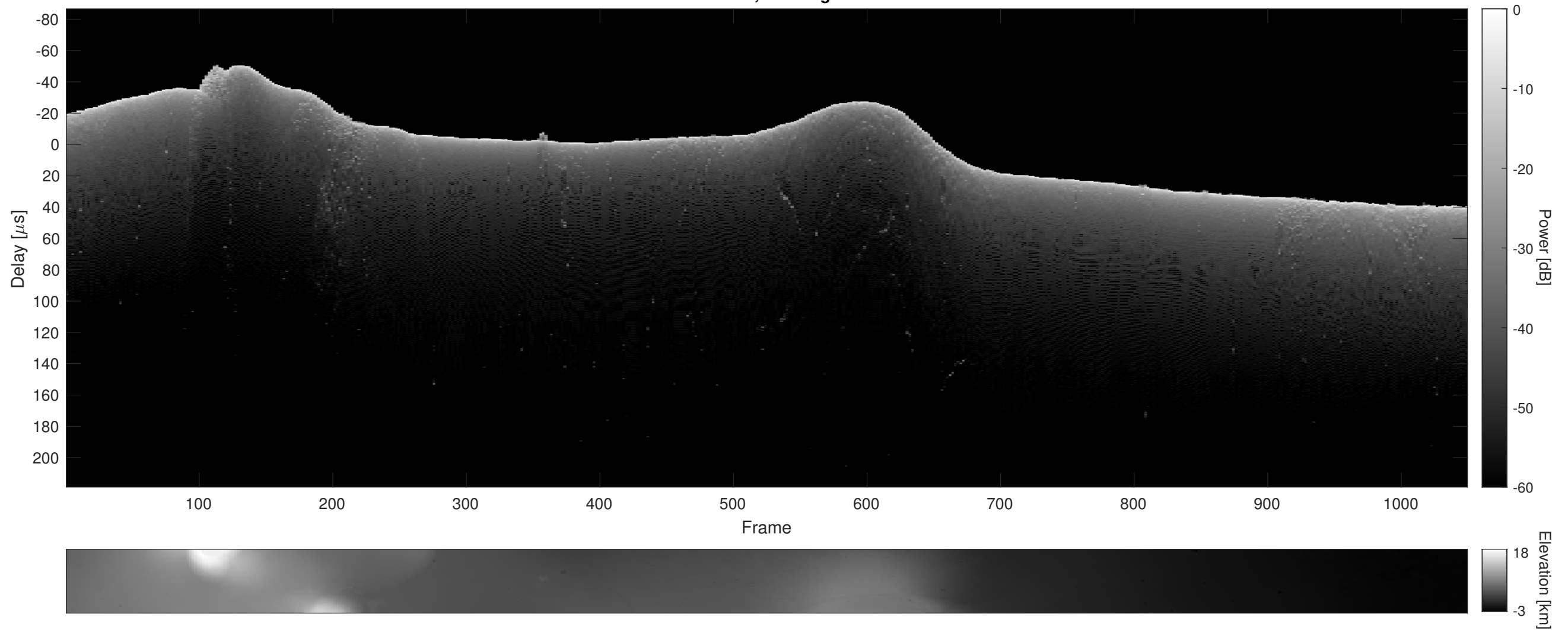
Orbit 8044, Cluttergram
