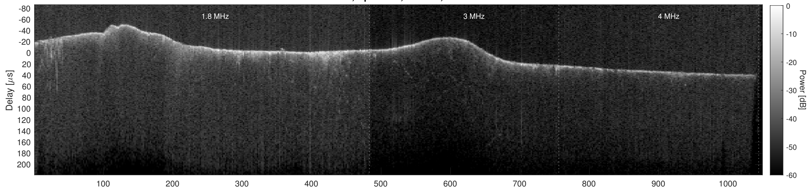
Orbit 8044, Cluttergram
