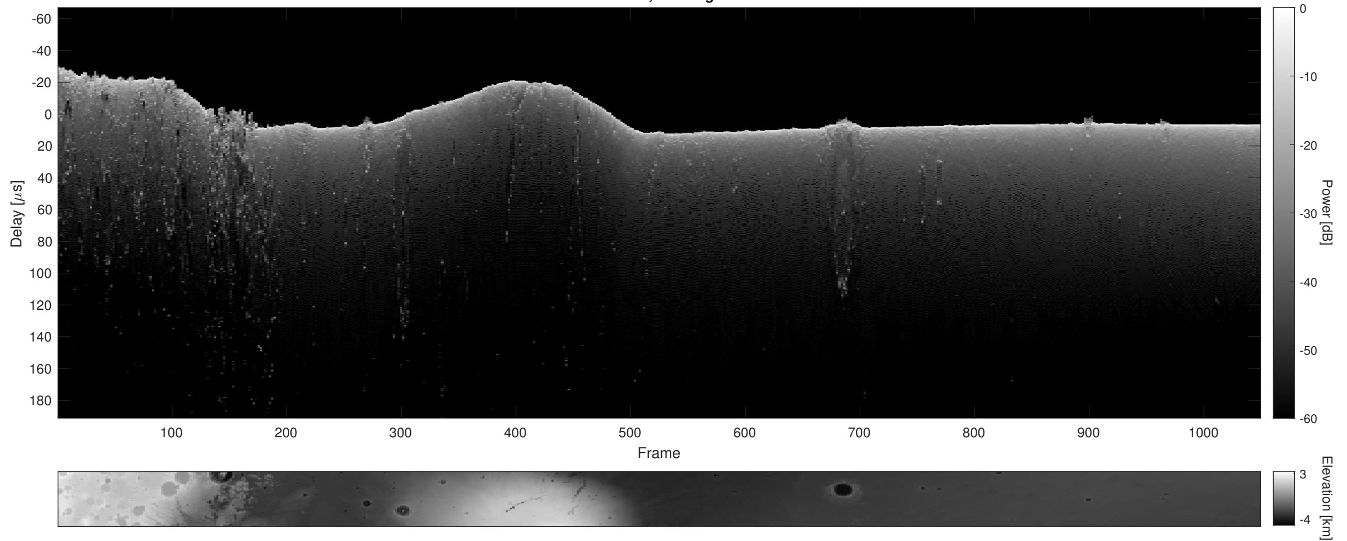
Orbit 8045, Cluttergram
