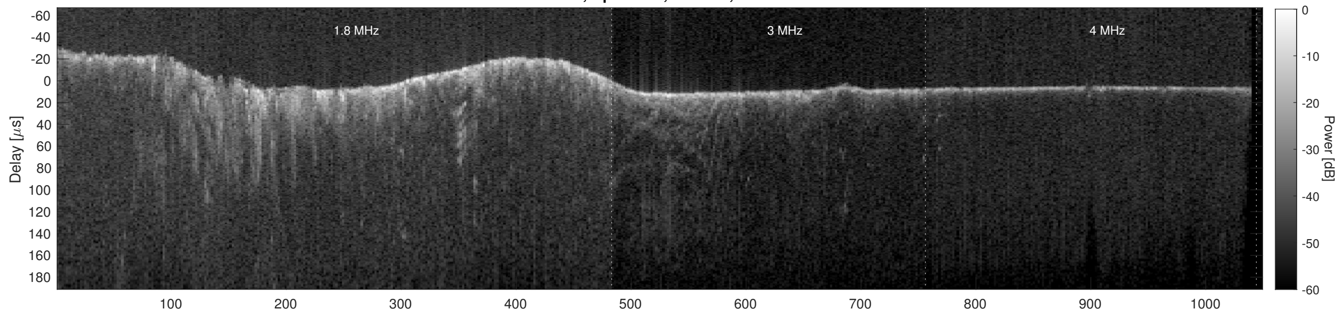
Orbit 8045, Cluttergram
