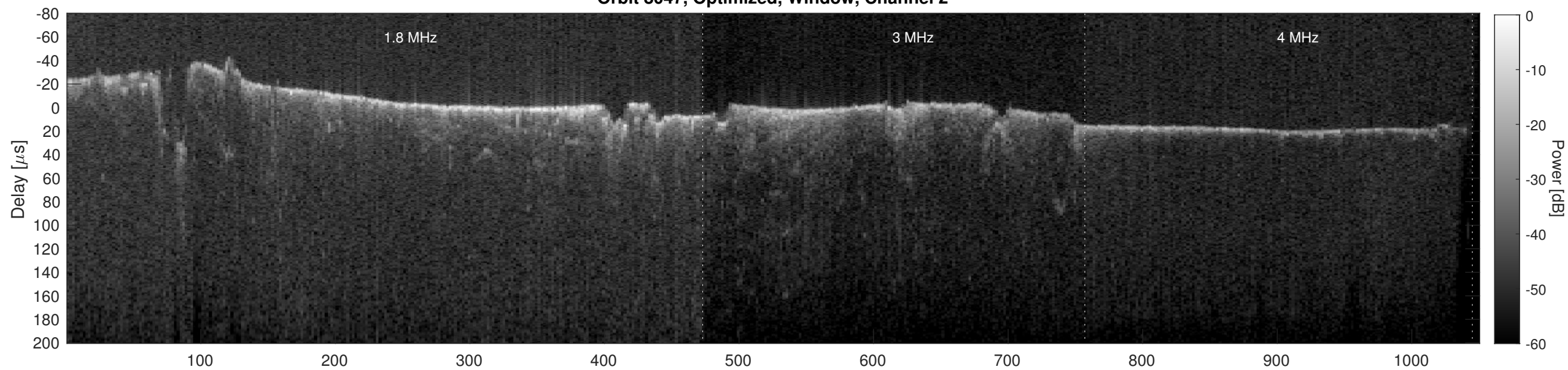
Orbit 8047, Cluttergram
