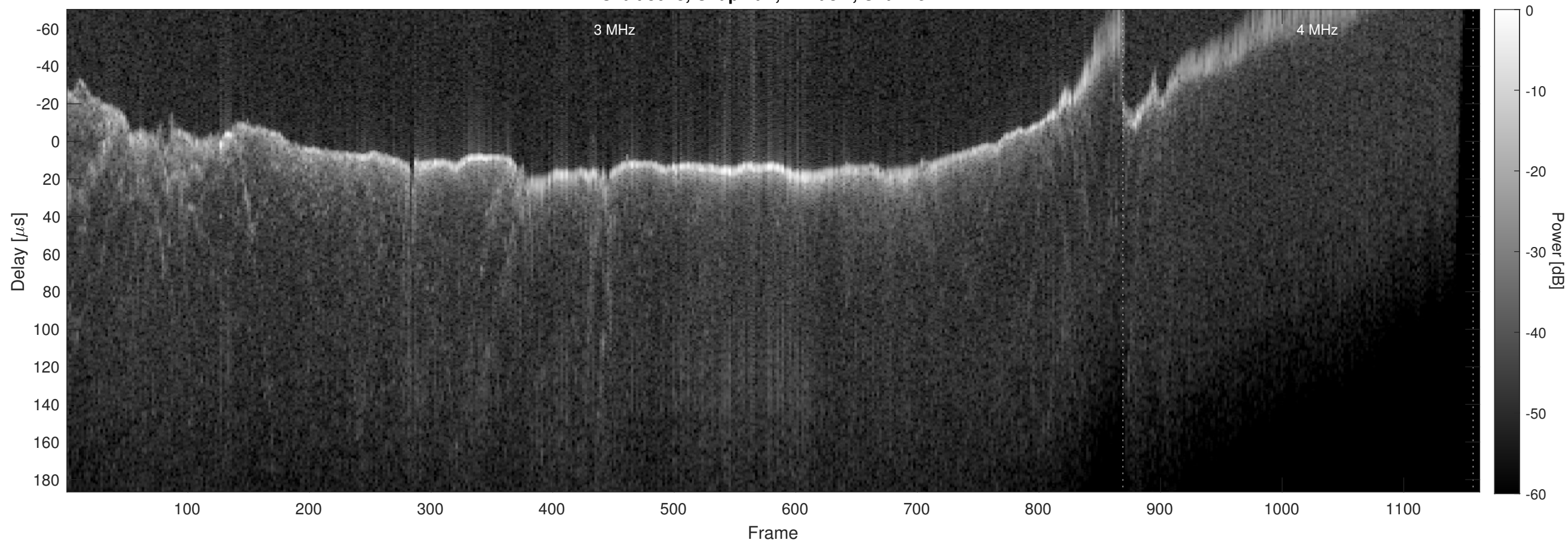
Orbit 8048, Chapman, Window, Channel 2
