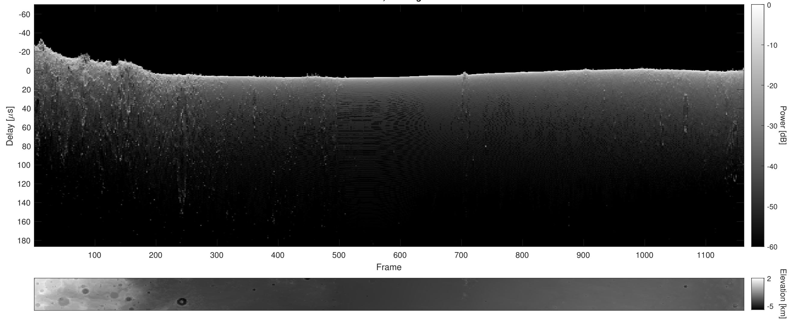
Orbit 8048, Cluttergram
