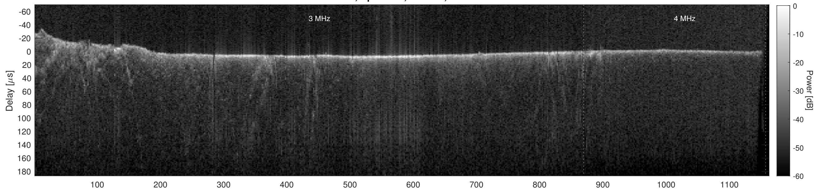
Orbit 8048, Cluttergram
