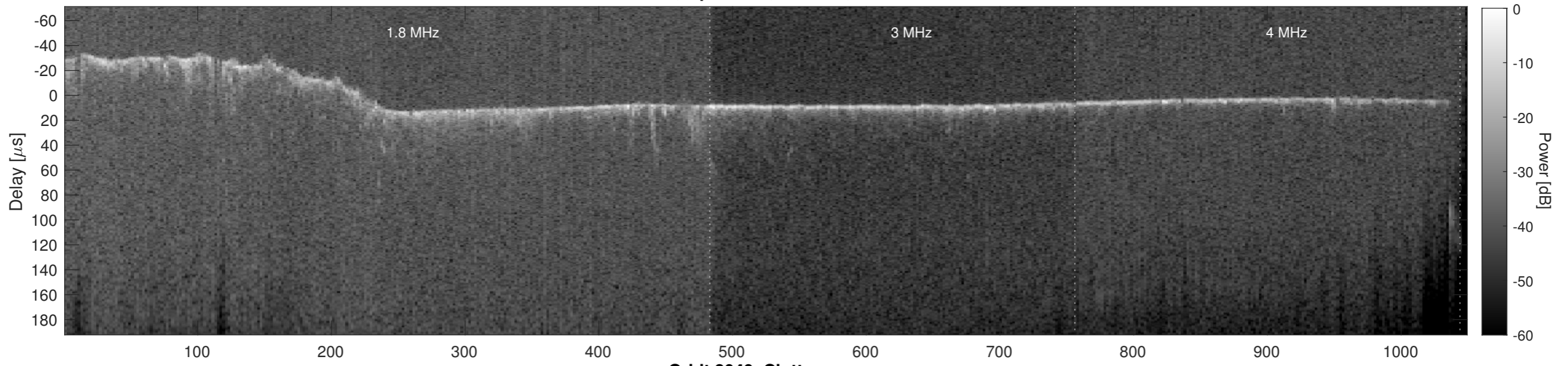
Orbit 8049, Cluttergram
