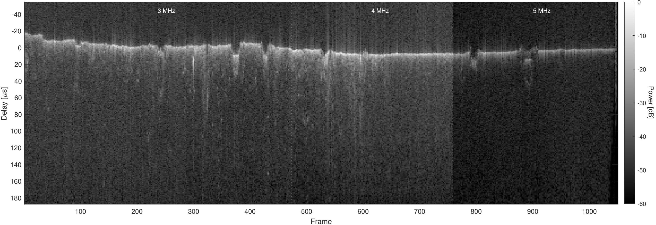
Orbit 8050, Optimized, No Window, Channel 2
