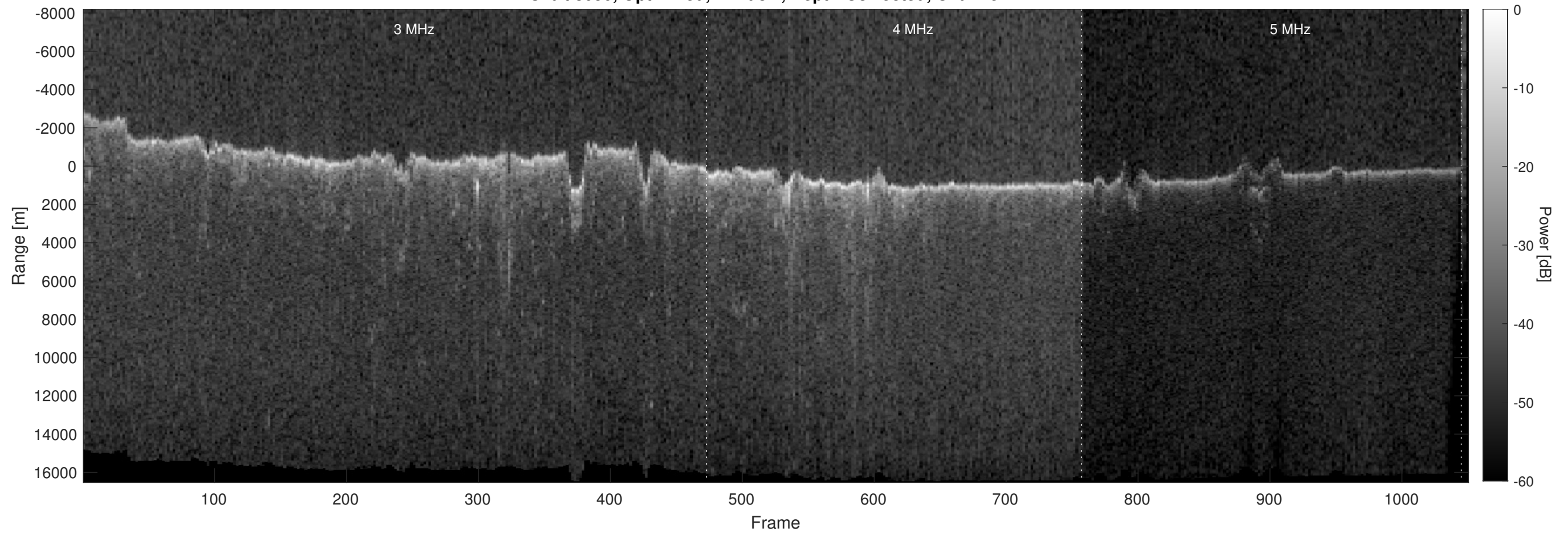
Orbit 8050, Optimized, Window, Depth-Corrected, Channel 2
