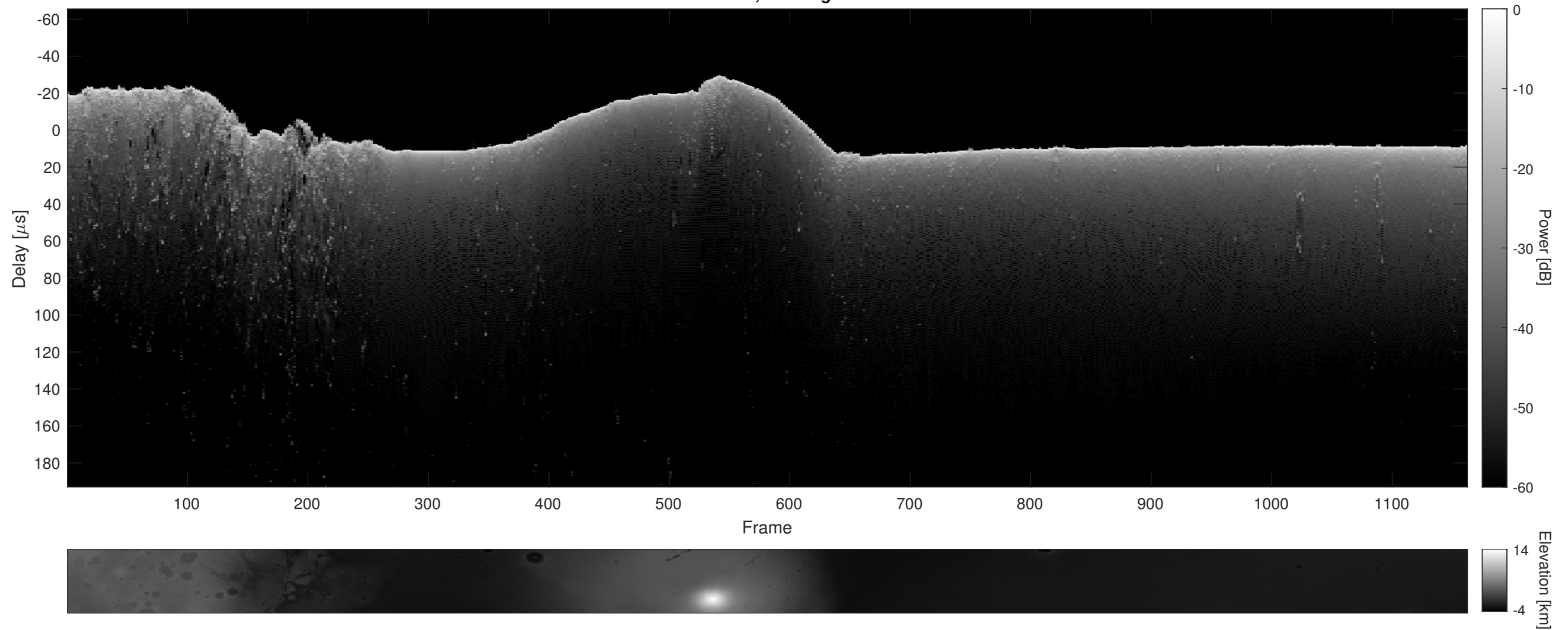
Orbit 8052, Cluttergram
