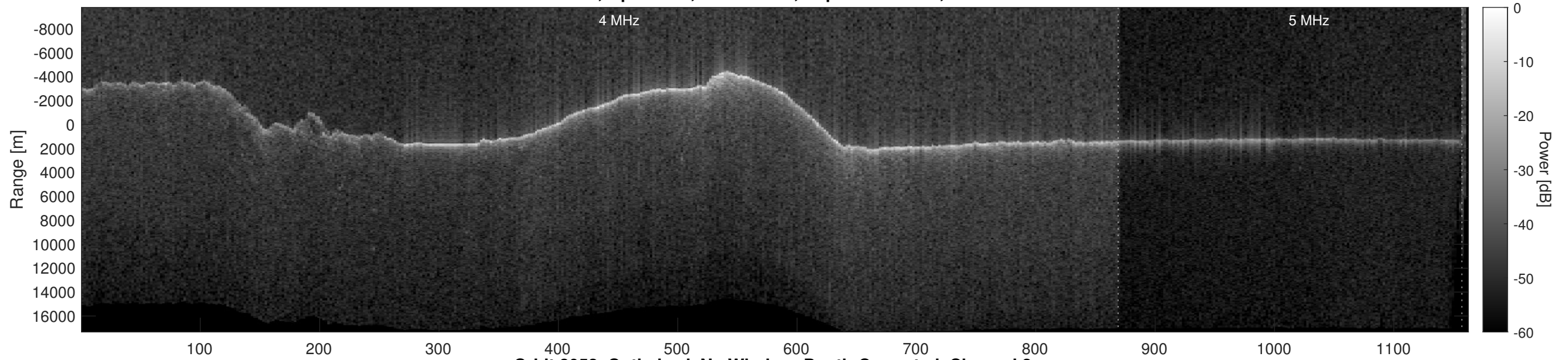
Orbit 8052, Optimized, No Window, Depth-Corrected, Channel 2
