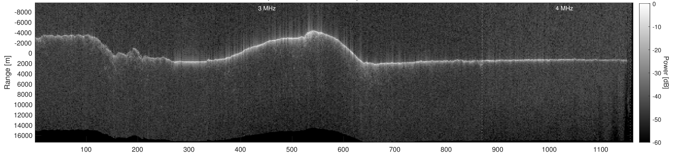
Orbit 8052, Depth-Corrected Cluttergram
