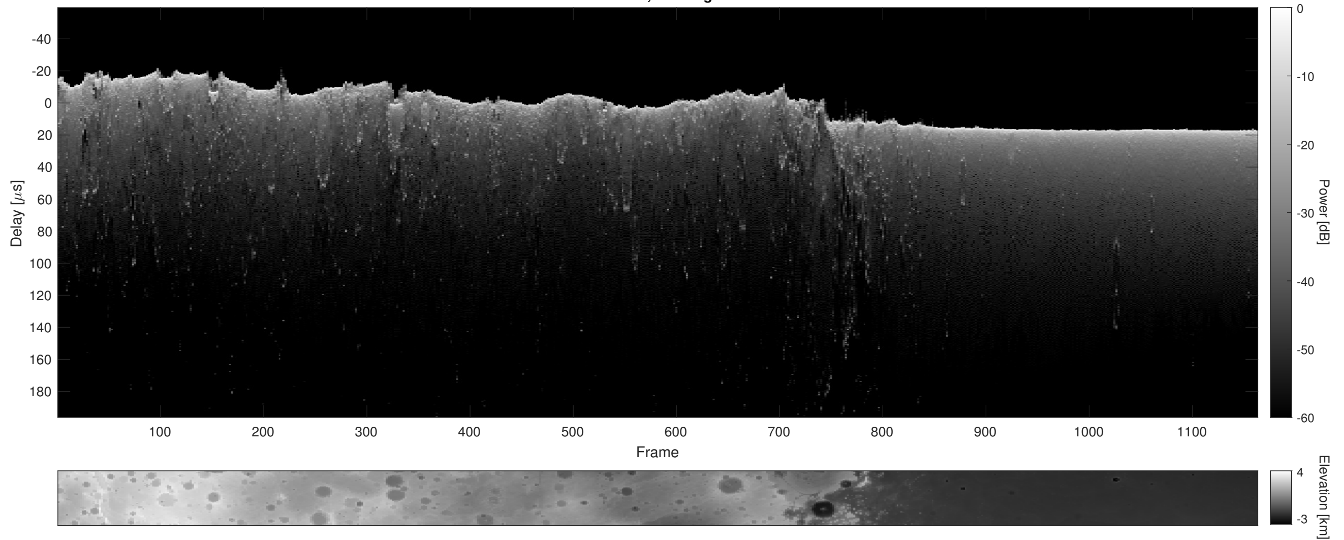
Orbit 8053, Cluttergram
