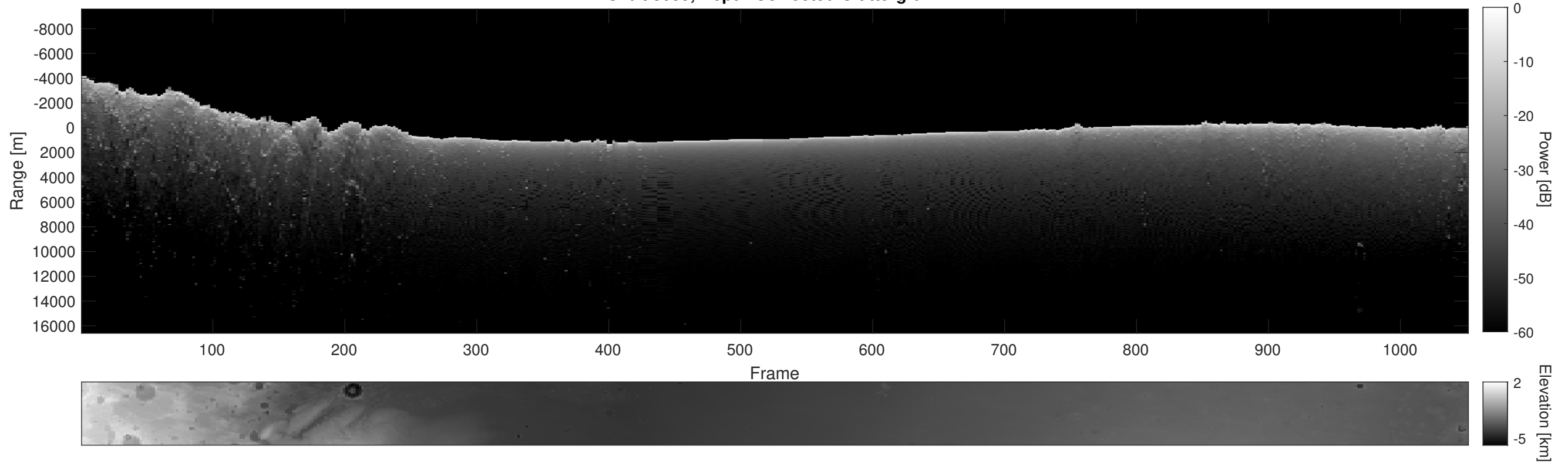
Orbit 8055, Depth-Corrected Cluttergram
