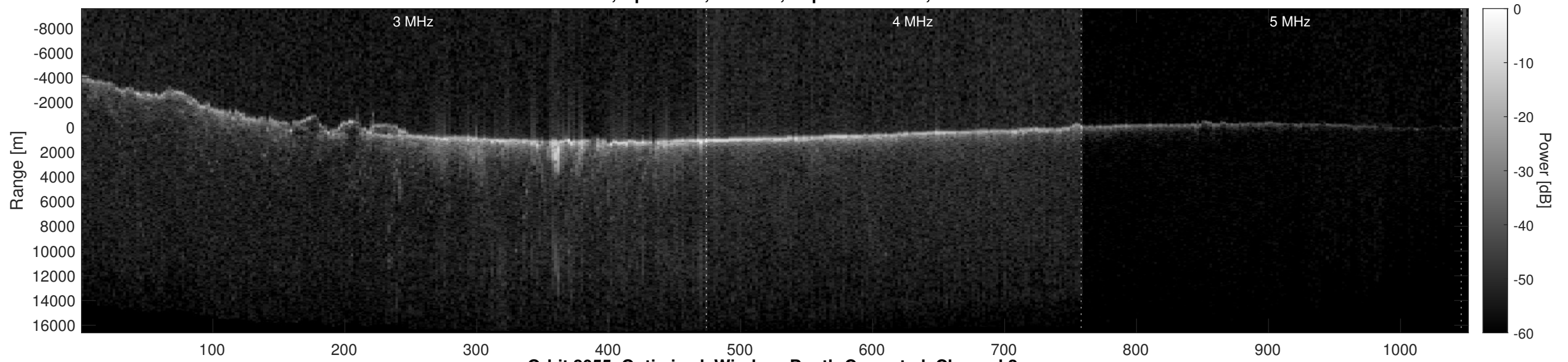
Orbit 8055, Optimized, Window, Depth-Corrected, Channel 2
