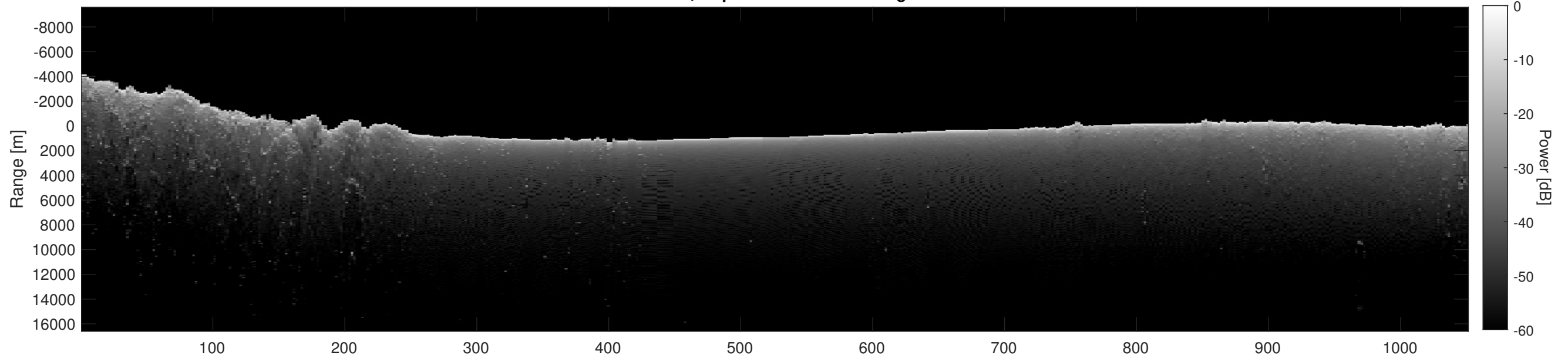
Orbit 8055, Depth-Corrected Cluttergram
