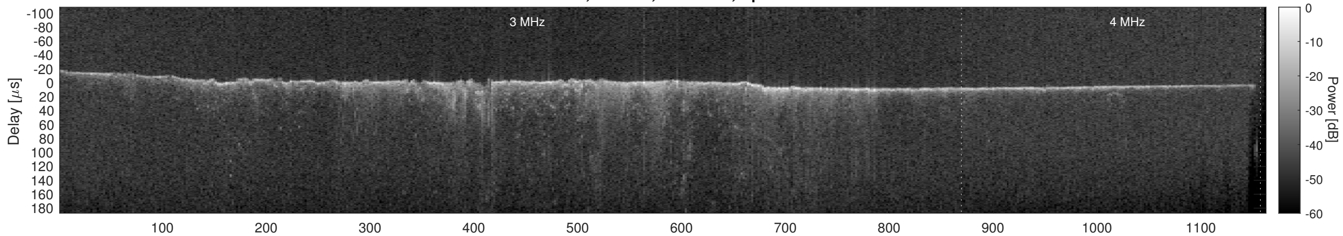
Orbit 8057, Cluttergram
