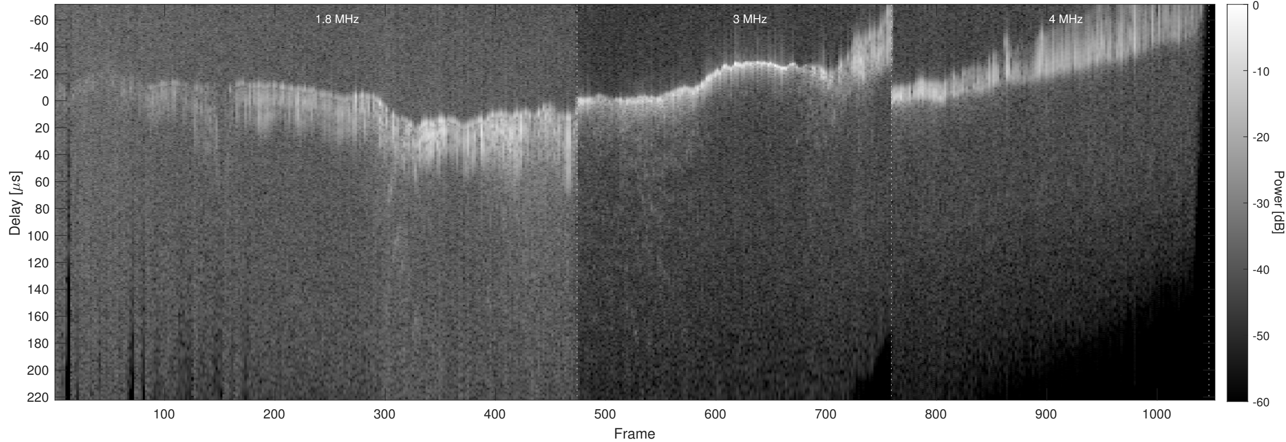
Orbit 8058, Chapman, No Window, Channel 2
