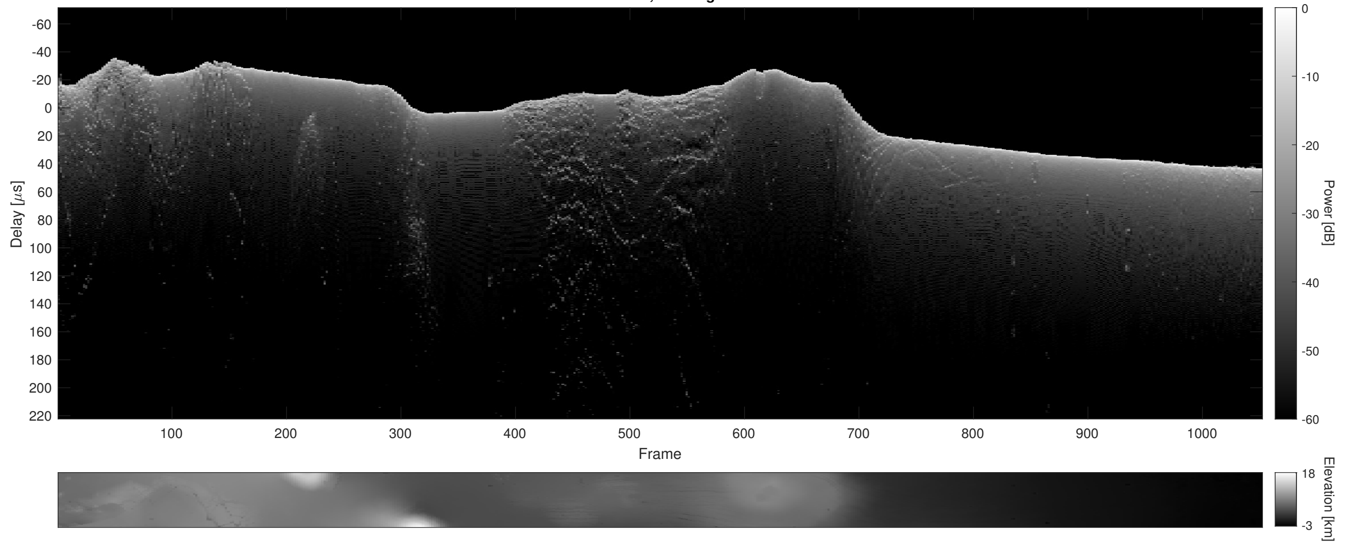
Orbit 8058, Cluttergram
