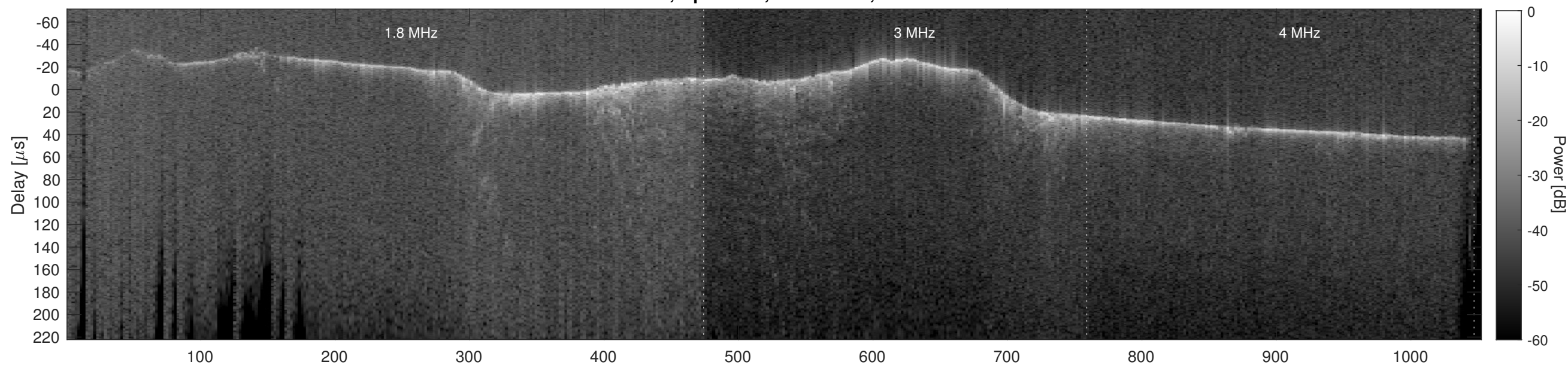
Orbit 8058, Cluttergram
