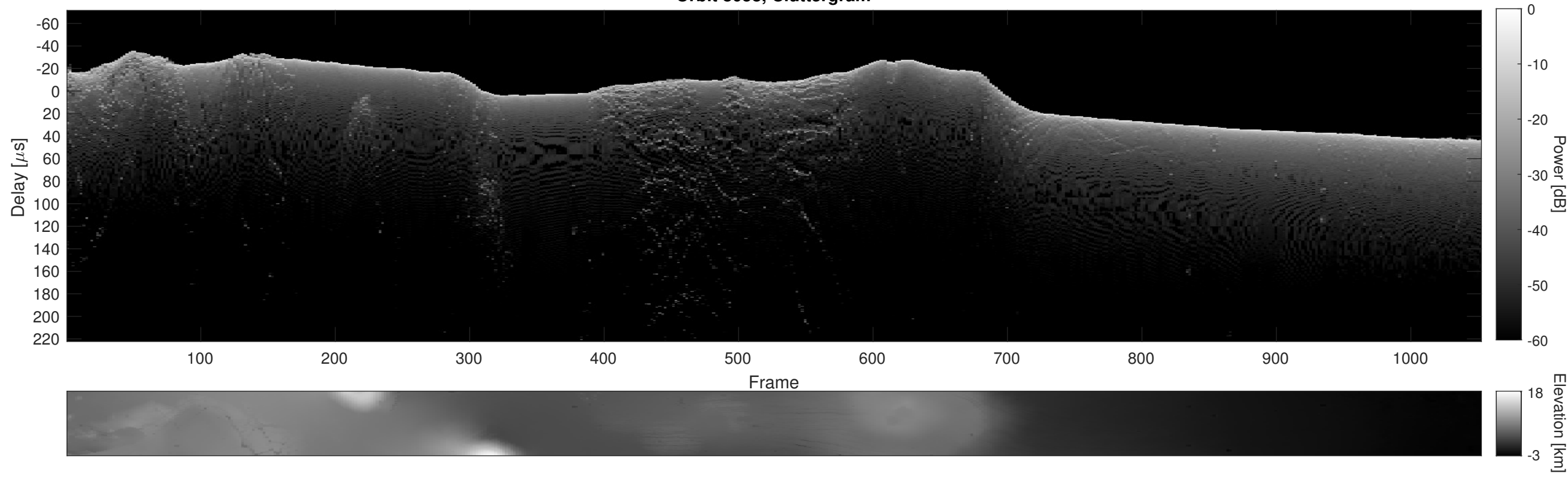
Orbit 8058, Cluttergram
