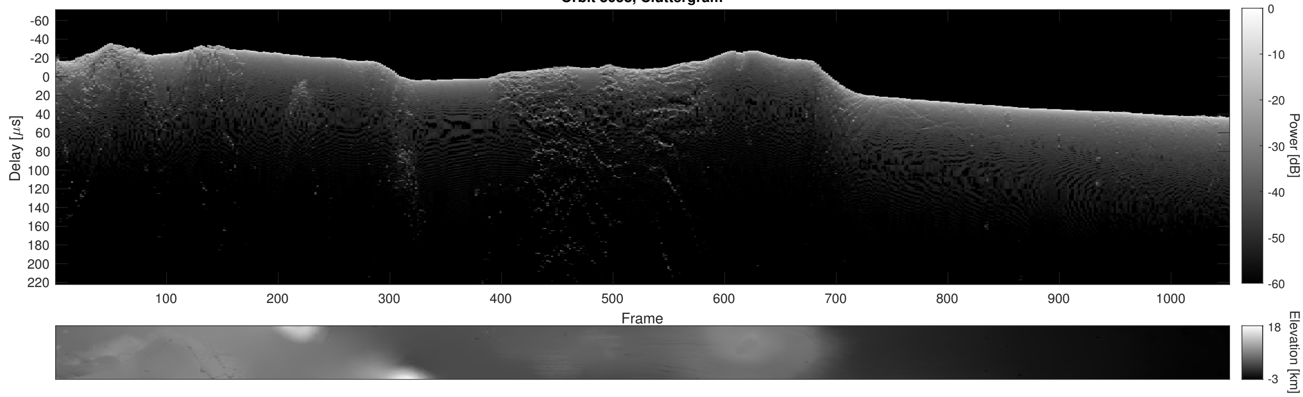
Orbit 8058, Cluttergram
