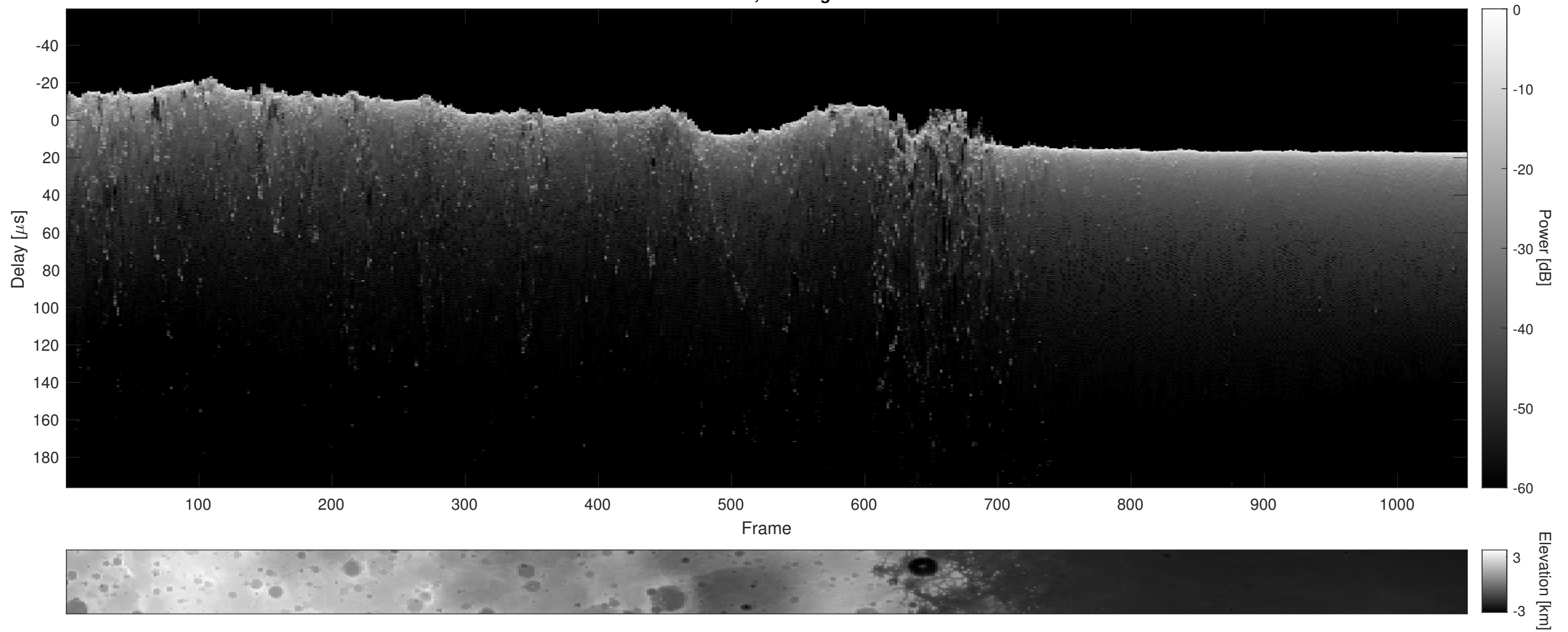
Orbit 8060, Cluttergram
