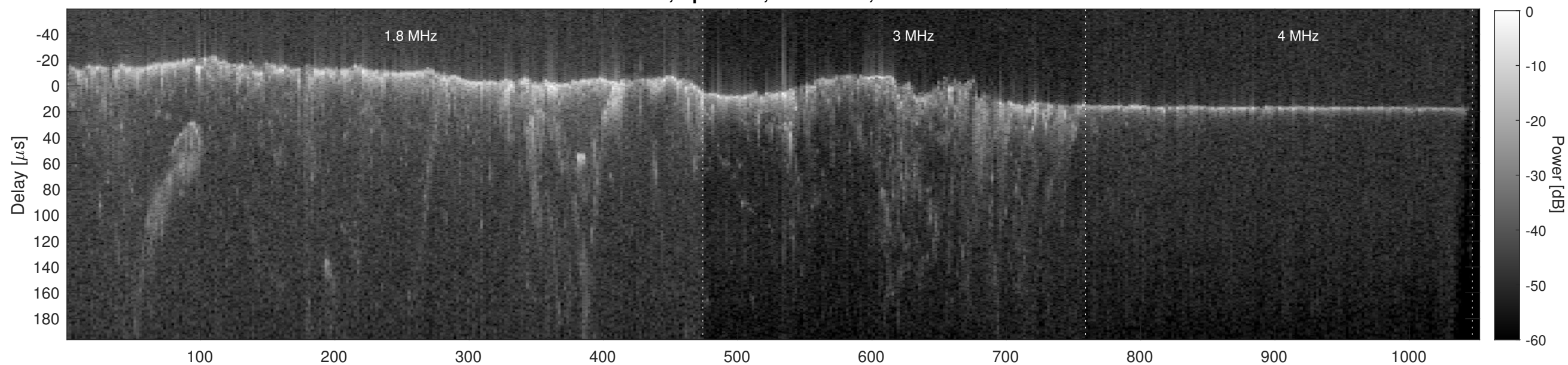
Orbit 8060, Cluttergram
