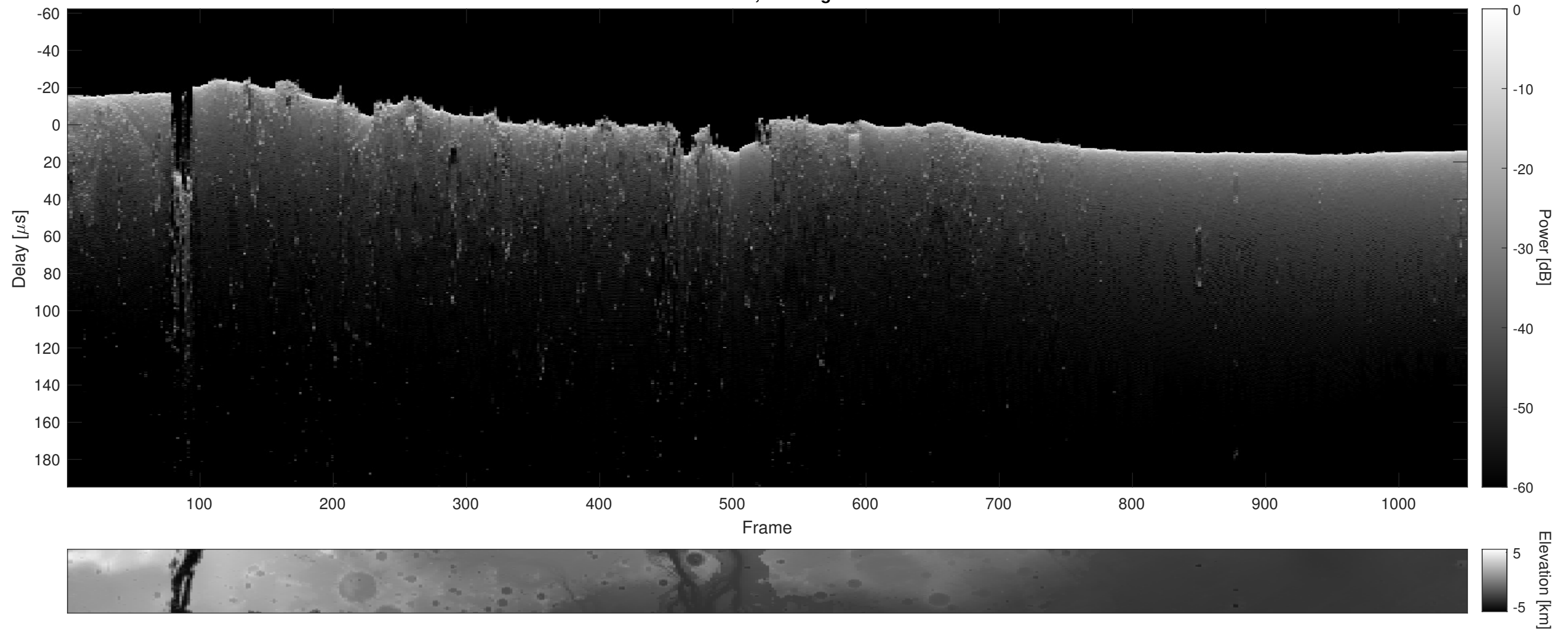
Orbit 8061, Cluttergram
