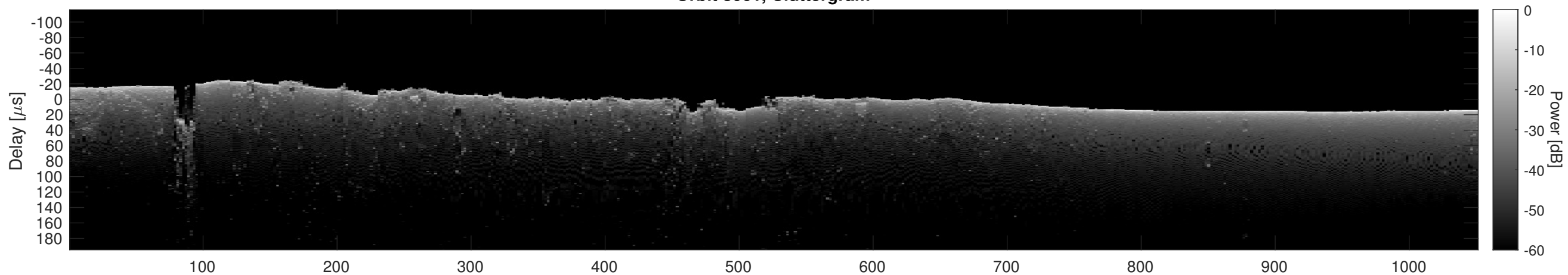
Orbit 8061, Cluttergram
