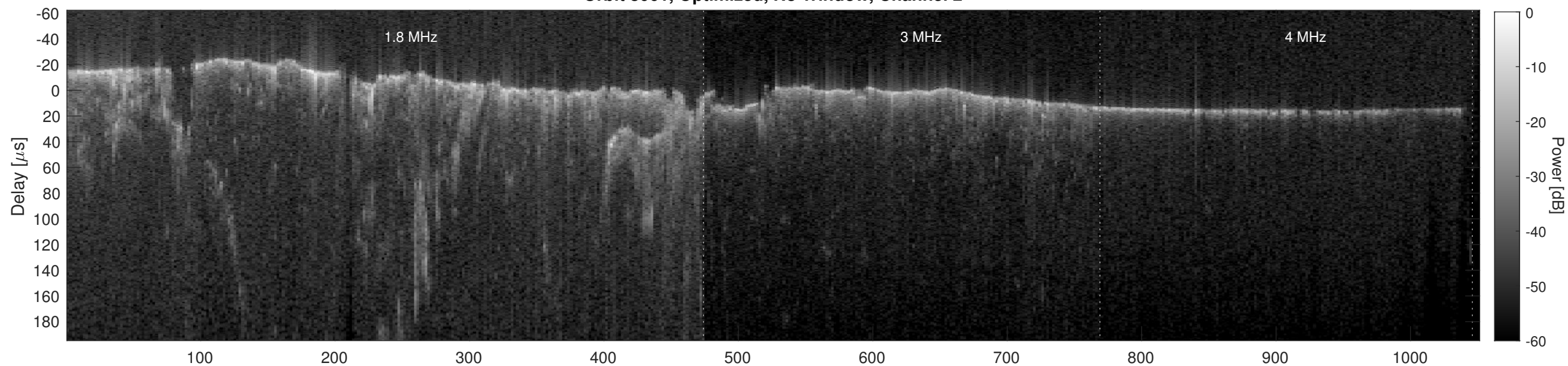
Orbit 8061, Cluttergram
