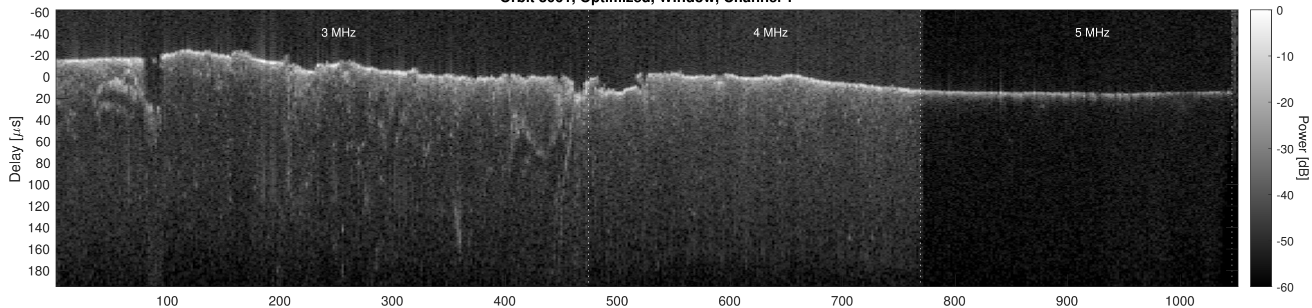
Orbit 8061, Optimized, Window, Channel 2
