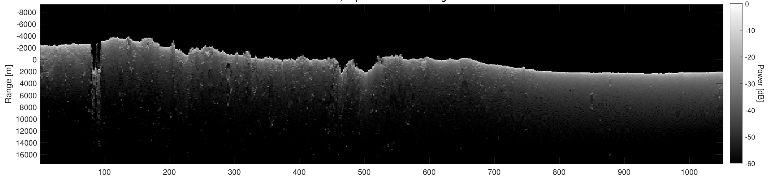
Orbit 8061, Depth-Corrected Cluttergram
